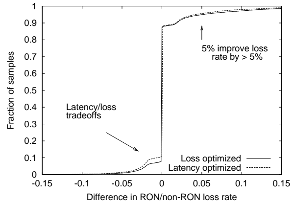
Figure 11: The cumulative distribution function (CDF) of the improvement in loss rate achieved by RON. The samples detect unidirectional loss, and are averaged over \tau = 1800 s intervals.
