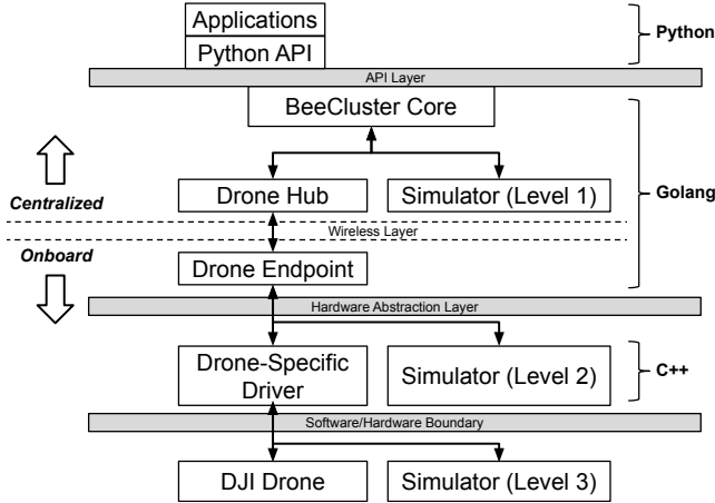
Figure 9: BeeCluster Framework
