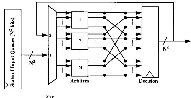
Fig. 22. Interconnection of N arbiters to implement iSLIP for an N \times N switch. Each arbiter is used for both input and output arbitration. In this case, each arbiter contains two registers to hold pointers g_i and a_i .
