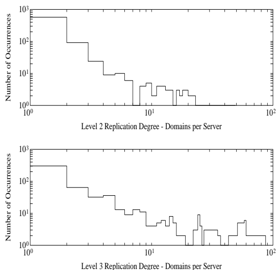
Figure 9: Number of DNS domains replicated on individual second and third level name servers.
