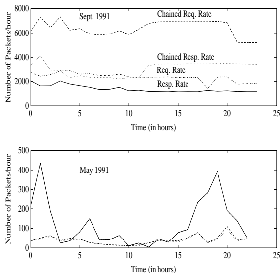
Figure 5: Request, response, and chained request and response rates at one of the other three name servers.
