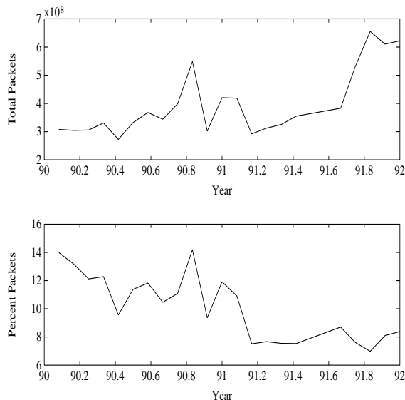
Figure 1: DNS contribution to NSFnet backbone packet counts for the past two years.
